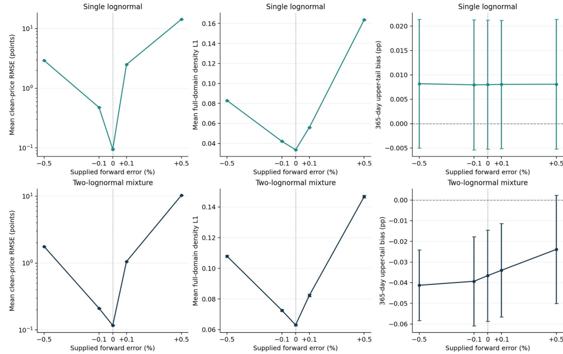
Figure 23. Sensitivity of the selected fit to the supplied forward, under Extended 121 coverage. Points are repetition means with \pm 2 MCSE; connecting lines are visual guides between the five stated stress levels. The price-error axis is logarithmic. The tail event remains S_T > 1.8 F_{true} at 365 days throughout. Calendar feasibility is checked separately in supplied-forward coordinates.
