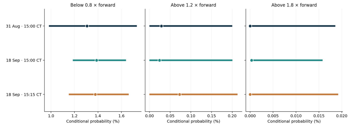
Figure 32. Dots are the minimum-curvature point estimates; horizontal bars are the conditional feasible probability ranges. Panels use different horizontal scales and percentages throughout. The bars are not statistical error bars. In particular, a nearly zero selected upper-tail probability can coexist with a materially positive feasible upper bound.
