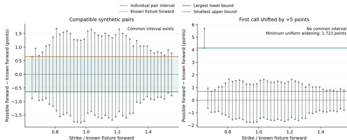
Figure 24. Conditional forward bounds for the first synthetic horizon. Each vertical segment is one call–put pair’s interval from Equation (8). The left panel has a common intersection. The right panel adds five points to the first call’s bid and ask while leaving the put unchanged; the largest lower bound then exceeds the smallest upper bound. The dotted line is the known fixture forward, available only because this example is synthetic. The shaded compatible band is not a confidence interval.
