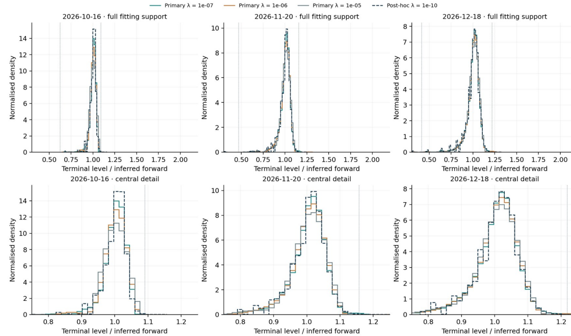
Figure 27. Market-density sensitivity to smoothing. The three solid curves use the declared primary coefficients; the dashed curve uses the post-hoc selected 10^{-10} . Top panels show the entire fitting support and lower panels enlarge 0.75 \leq S/F \leq 1.25 . Dotted vertical lines delimit the retained strike range. Curves are estimated histograms, not analytical benchmark densities. Tiny far-tail masses are easier to compare numerically in Table 30 than on this peak-dominated linear scale.
