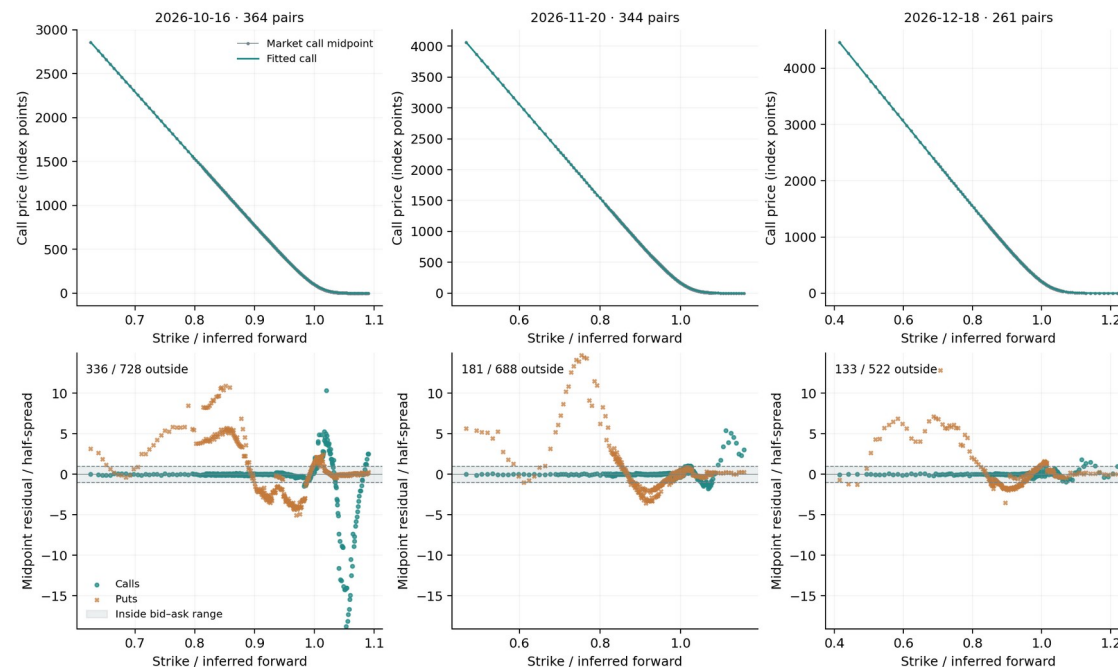
Figure 26. Primary market fit and bid-ask residuals on 18 September 2026. Upper panels show market call midpoints and the selected fitted call curve. Lower panels show both option types in units of their own half-spread. The shaded band is the bid-ask interval. The common vertical range covers every residual; misses are retained rather than clipped. Prices are index points, not dollars per contract. All retained spreads in this case have positive width.
