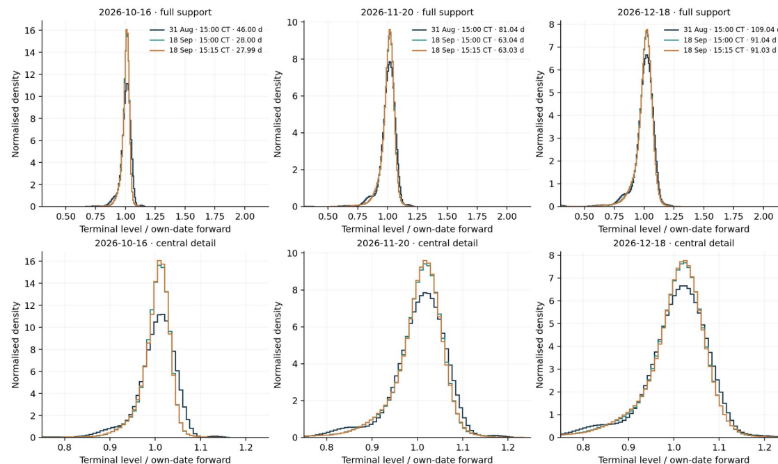
Figure 30. Fixed-expiry density comparisons, with full support above and central detail below. The elapsed horizon falls by 18 days between August and standard September, and by another 15 minutes at the later snapshot. Each curve uses its own inferred forward; the same normalised threshold can therefore correspond to different index levels. These curves cannot isolate a pure change in expectations at a fixed horizon.
