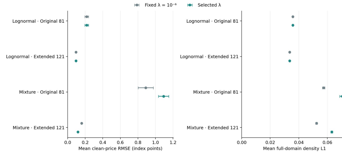
Figure 22. Mean clean-price RMSE and full-domain density error after refitting with selected or fixed smoothing, using the same quote realisations in each comparison. Bars show \pm 2 MCSE. A small price error does not, by itself, establish a small density error, since prices integrate the density through the payoff relationship in Equation (1).
