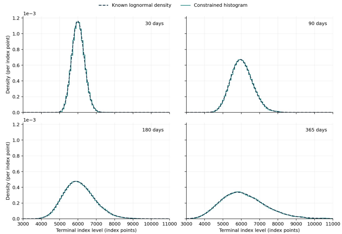
Figure 11. Known lognormal densities and fitted histogram slices at 30, 90, 180 and 365 days. All panels use the same axes. The stepwise density is the actual interval representation, without display smoothing. The interactive companion permits selection of all eight fitted horizons.
