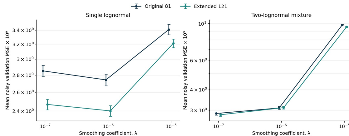
Figure 21. Mean pooled noisy-price validation MSE for each smoothing coefficient, with \pm 2 Monte Carlo standard errors across the 20 repetitions. The dimensionless score is multiplied by 10^9 for display and the vertical scale is logarithmic. Lines connect the three evaluated candidates. These scores select the coefficient; they are not the final recovery-performance estimates.
