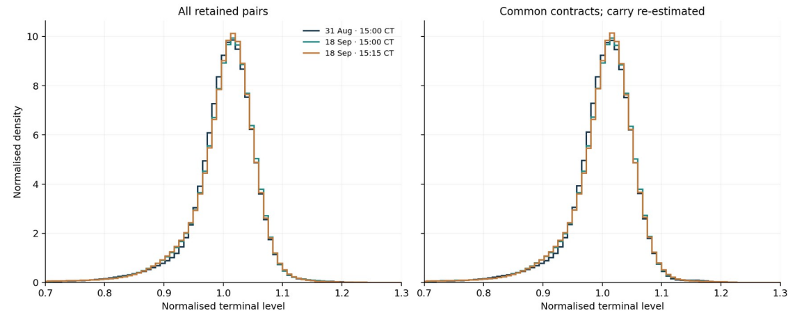
Figure 31. Interpolated 60-day normalised density using all retained pairs, and the separately re-estimated common-contract control. The panel displays 0.7–1.3 for detail; the fitted support remains 0.3–2.2, and tail calculations use the complete support. The right panel changes both quote composition and inferred carry.
