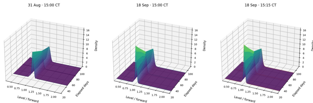
Figure 33. The three fitted surfaces on common normalised-level, elapsed-day and density scales. Only three expiry densities are fitted in each snapshot. Surface joins between bin centres and maturity rows aid viewing; they are not extra observations. The companion adds rotation, zoom, hover, observed-snapshot playback, exact histogram slices and the separately labelled 60-day mixture.
